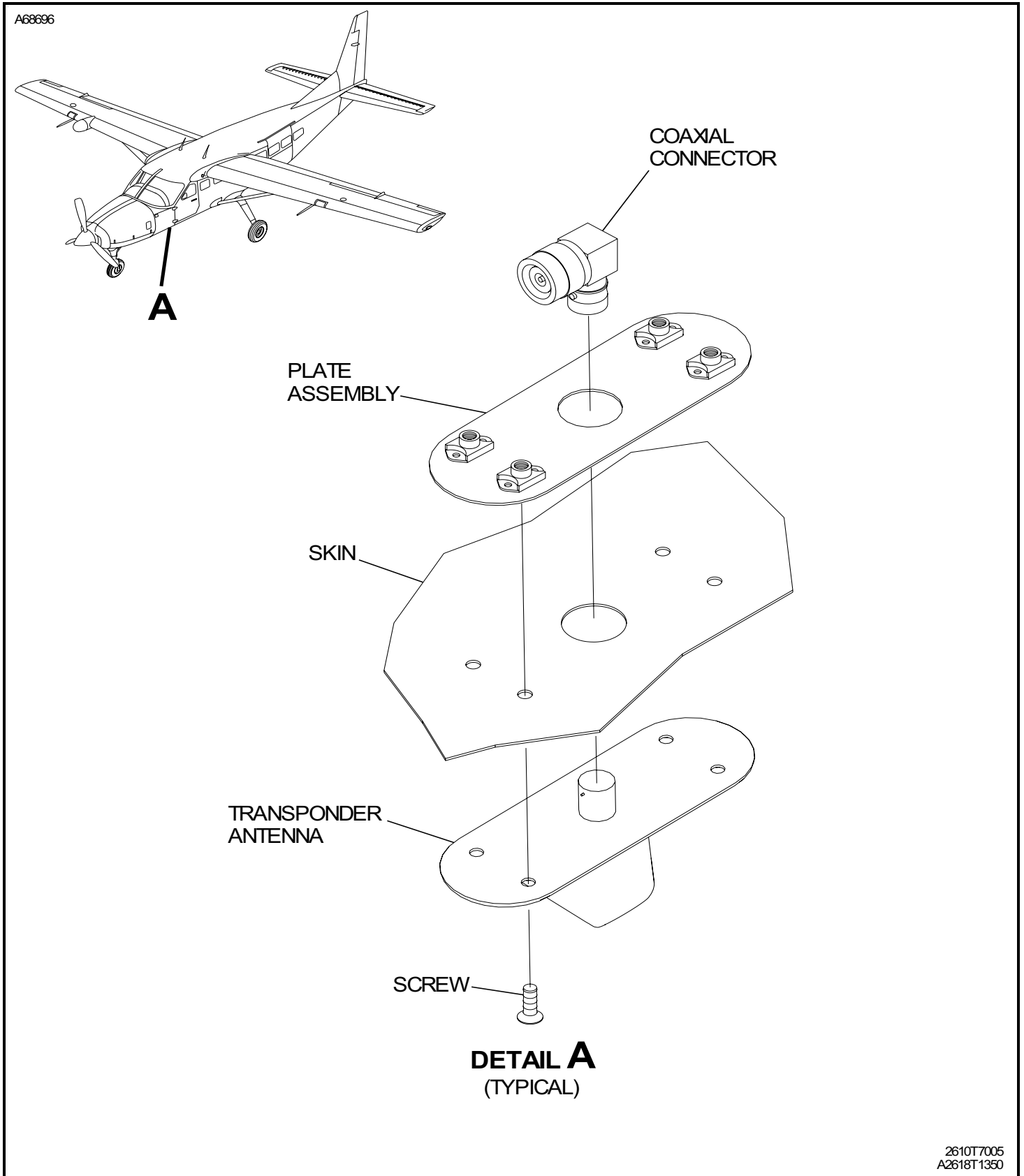
Figure 401 : Sheet 1 : Transponder Antenna Without Cargo Pod
