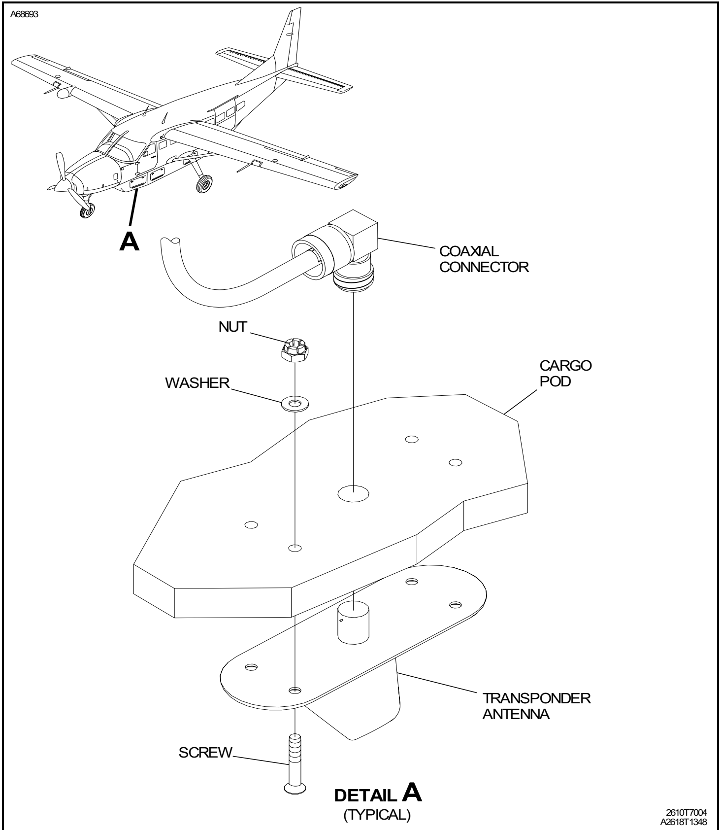
Figure 402 : Sheet 1 : Transponder Antenna With Cargo Pod
